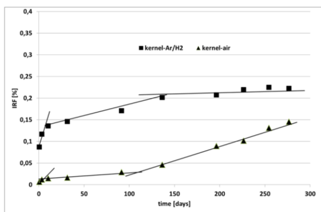
Figure 2: FIAP ^{90}\text{Sr} (%) vs. time under oxic and under anoxic/reducing conditions.
