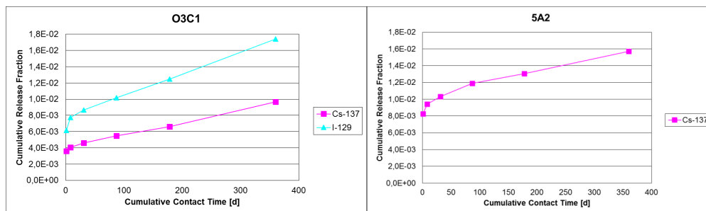
Figure 4: Release rates of 137 Cs and 129 I sample C1 and 5A2.
