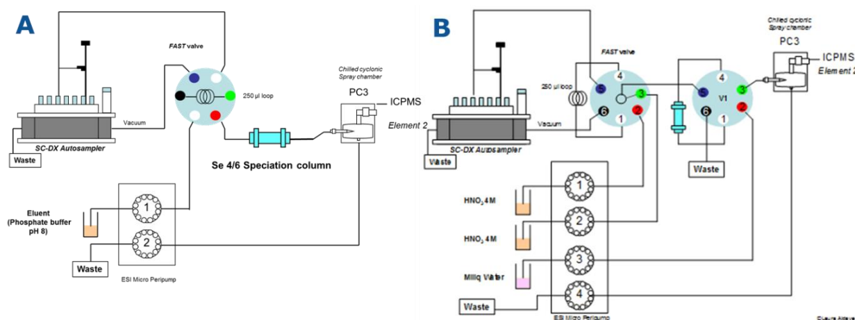
Figure 1: (A) FAST system configurations for speciation analysis (A) and for pre-concentration and/or separation (B) purposes.
