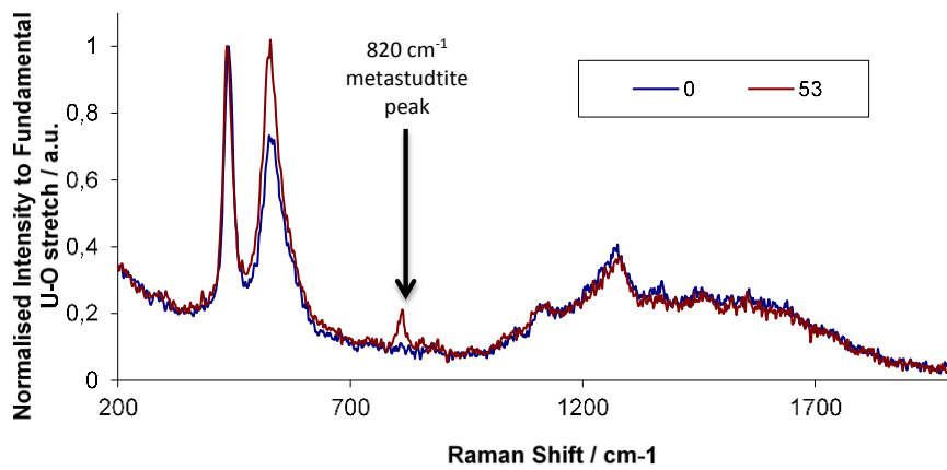
Figure 4: Raman Spectroscopy of a 25 GWd/tU SIMFUEL after 0 and 53 hours exposure to anoxic solution of 1mmol dm -3 H 2 O 2 , showing metastudtite formation at 820 cm -1 after 53 hrs exposure.
