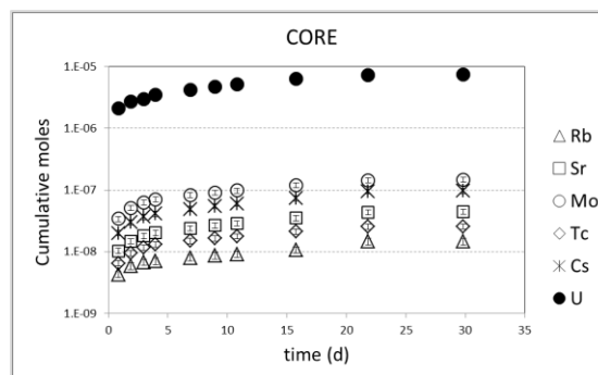
Figure 6: Measured cumulative moles as a function of time for the CORE powder experiment.
