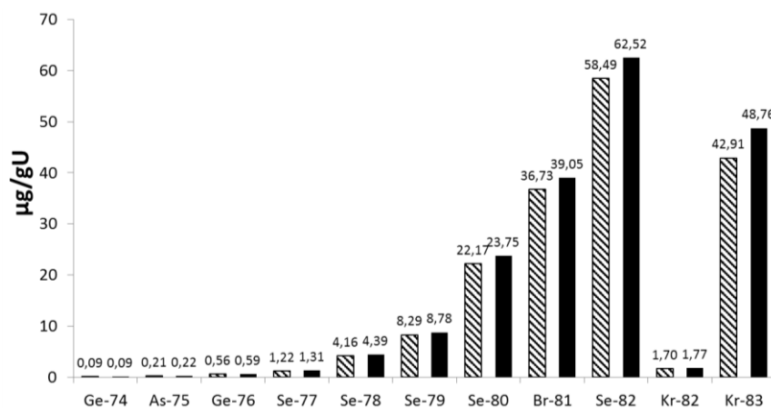
Figure 1: Origen calculated inventory for the 5A2 (diagonal) and C1 (solid) fuel samples.
