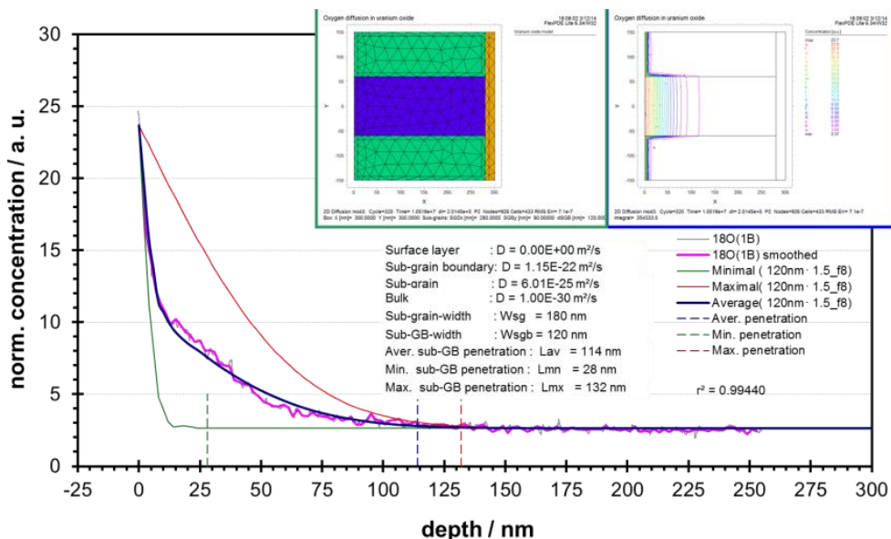
Figure 9: Two parallel 18 O diffusion processes in UO 2 where identified.
