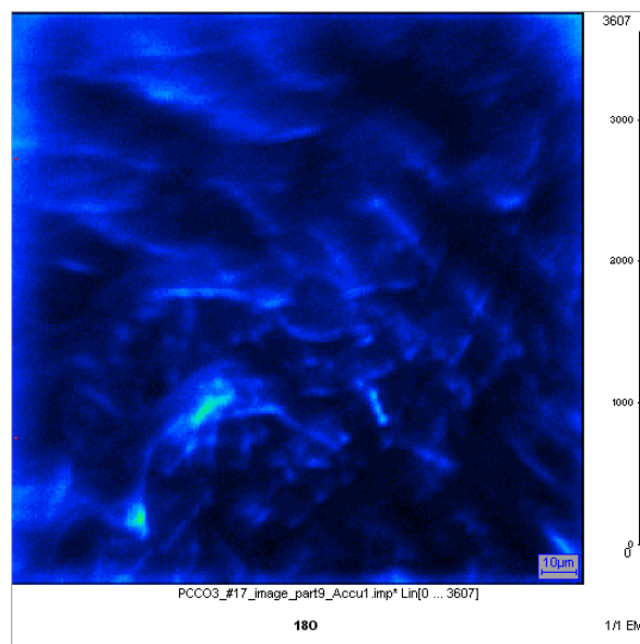
Figure 4: Ion filtered image at the nominal depth of 15 nm shows non-uniform distribution of ^{18}\text{O} .
