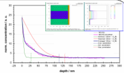
Figure 3 Two parallel 18 O diffusion processes in UO 2 where identified.
