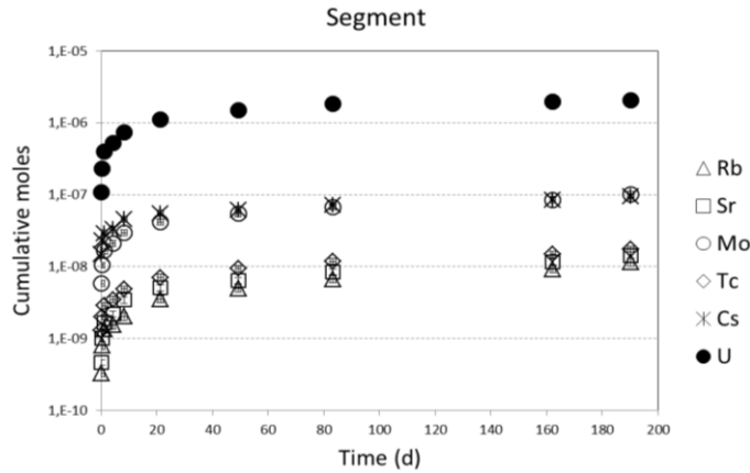
Figure 3: Elemental cumulative moles vs time. Experiment carried out with segment.
