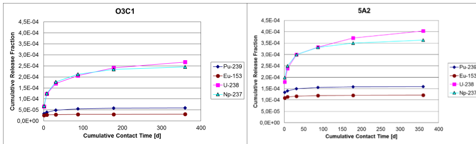
Figure 7: Release rates of 239 Pu, 153 Eu, 238 U and 237 Np sample C1 and 5A2.
