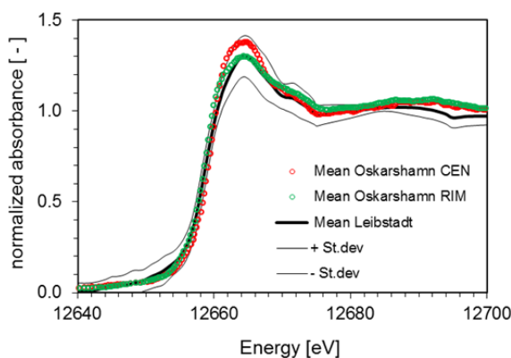
Figure 6: Averaged Se K-edge micro-XANES spectra from the central and peripheral regions of a spent fuel pellet from the Oskarshamn-3 reactor compared to the averaged spectrum ( \pm standard deviation) measured on spent fuel from the Leibstadt reactor.
