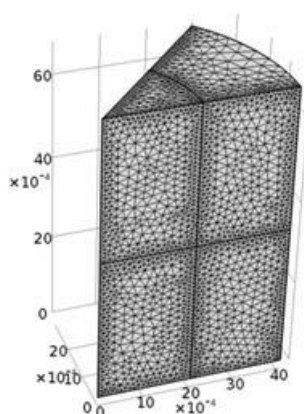
Figure 3: The geometry and finite element mesh of the 1/16 th fragment of the Reference Pellet for which calculations were performed. Dimensions are in metres.
