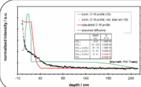
Figure 2 Modelling using variable diffusivity from published oxygen diffusivities of different uranium oxides.
