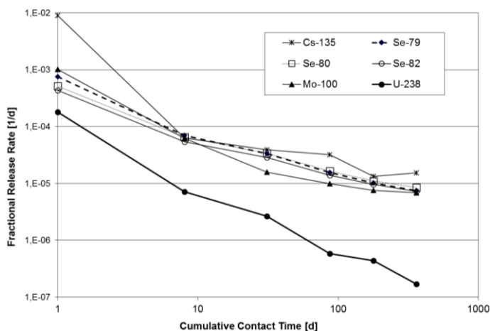
Figure 3: Release rates of 79 Se and selected radionuclides from the fragment leaching of sample 5A2.
