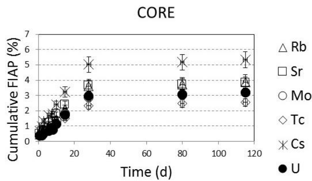
Figure 7: Cumulative FIAP(%) vs time. Experiment carried out with powder from the centre (CORE) of the SNF.
