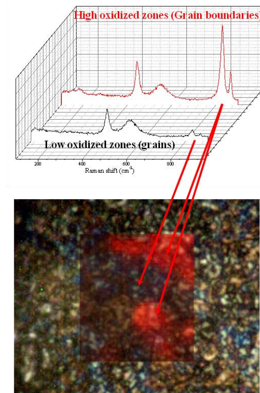
Figure 5: Space-resolved Raman spectra of corroded UO_2 with GB (red) and Grains (black).
