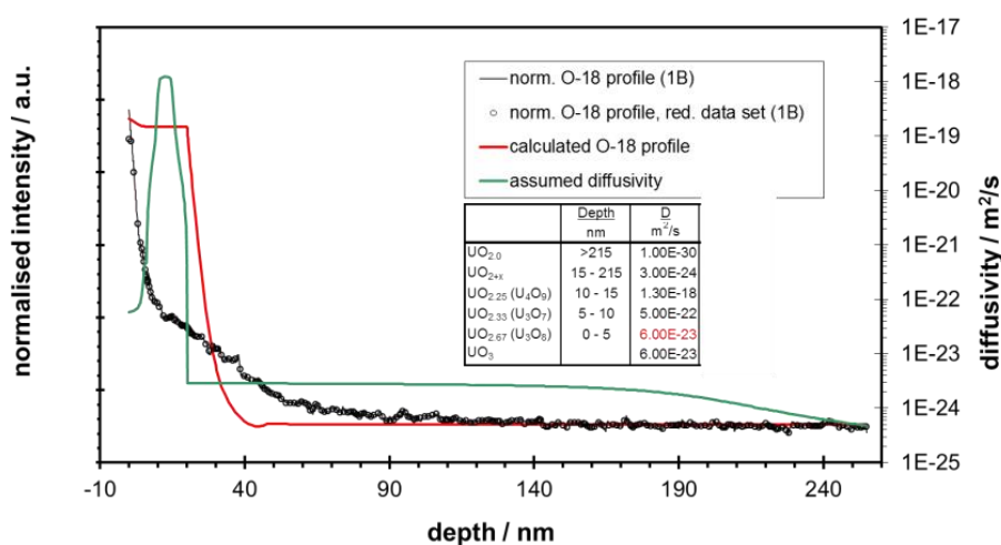
Figure 8: Modelling using variable diffusivity from published oxygen diffusivities of different uranium oxides.
