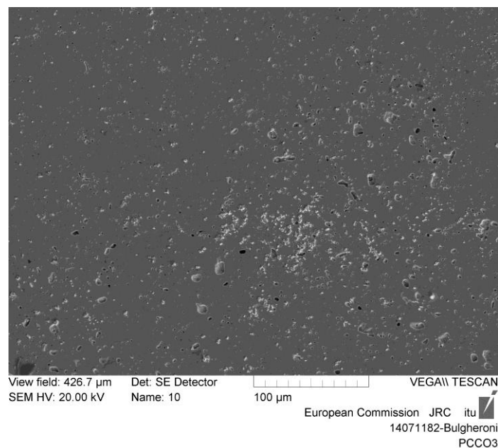
Figure 6: SEM image of a sample region containing a shallow crater.
