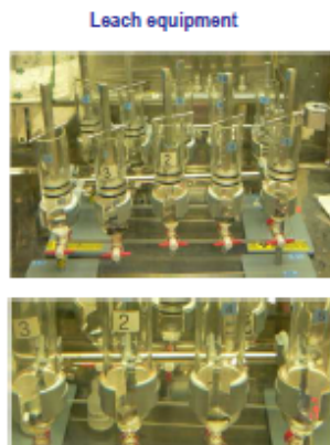
Fig. 1: Assembly of glass columns used for the PSI leach experiments. Bottom: BNF samples before introducing the aqueous solution. Top: 4 th operation, after filling with solution (pre-leaching step).
