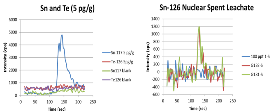
Figure 4: (Left) Behaviour of Sn and Te in the chelating column. (Right) Detection of ^{126}\text{Sn} in nuclear spent fuel leachates (dilution 1/10).
