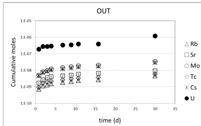
Figure 7: Measured cumulative moles as a function of time for the OUT powder experiment.
