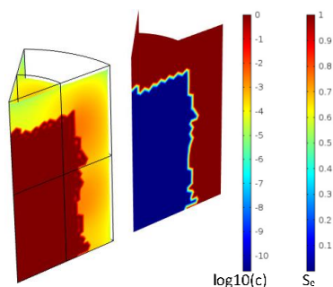
Figure 5: Tracer concentration ( \log_{10}[\text{mol/L}] – left) and saturation with water ( S_e – right) calculated at time 3 hours in “macro cracks” of the (1/16 th ) fragment of the pellet.
