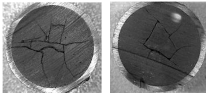
Figure 1: Cross sections of spent fuel sample used in leaching experiment.
