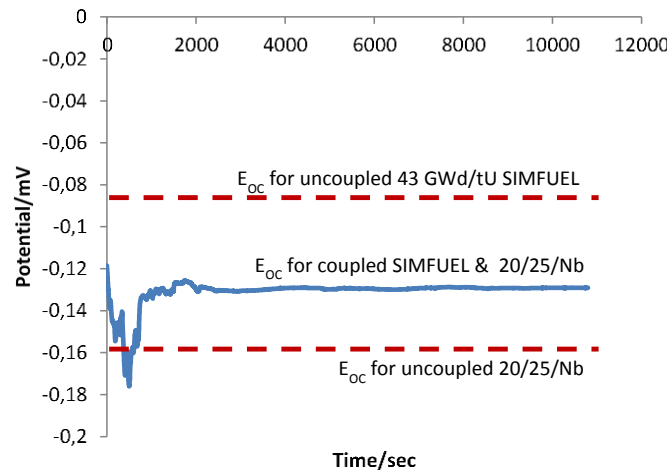
Figure 5: Open Circuit Potential of coupled 43 GWd/tU & 20/25/Nbvs time in anoxic modified simplified Groundwater.
