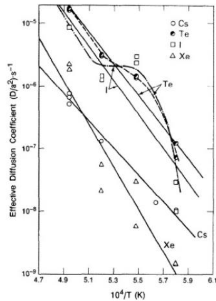
Figure 3: Effective diffusion coefficients for the volatile fission products in trace-irradiated sintered UO_2 . Systematic counting uncertainties range from about 3% (Te) to 20% (Xe).
