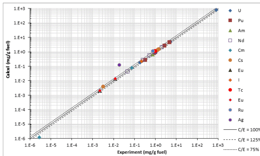
Figure 2: Comparison between the calculated radionuclides concentrations in the fuel and their measured concentrations by radiochemical analysis.
