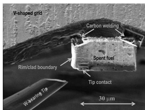
Figure 2: FIB Sample (“RIM”) of Oskarshamn spent fuel for XANES measurements (courtesy Studsvik Nuclear AB).
