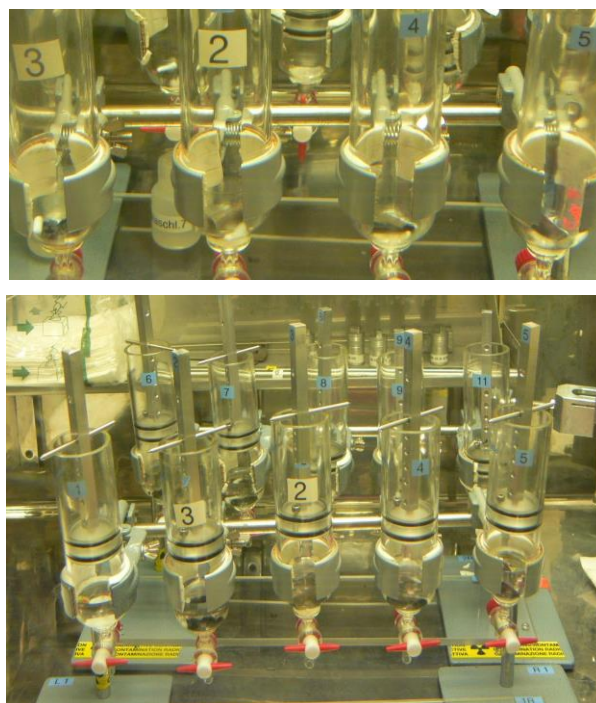
Figure 1: Assembly of glass columns used for the PSI leaching experiments. Top: SNF samples before introducing the leaching solution. Bottom: columns “in operation”, after filling with leaching solution.
