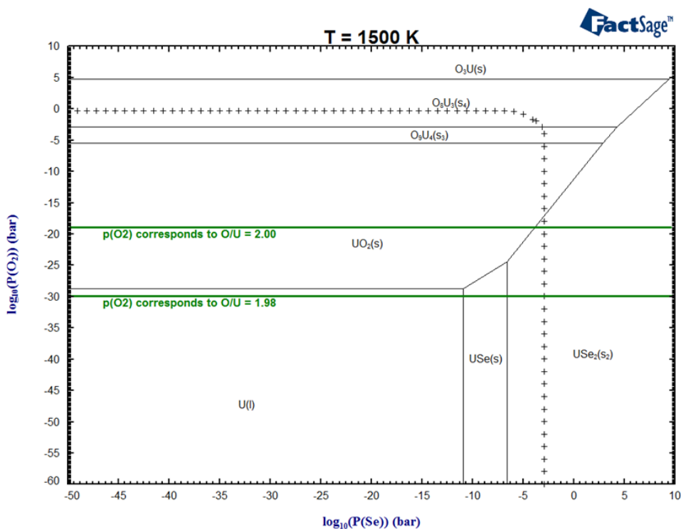
Figure 3: Predominance phase diagram of the Se-U-O system calculated for 1500 K.
