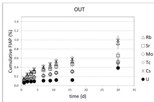
Figure 11: Cumulative FIAP as a function of time for the OUT powder experiment.
