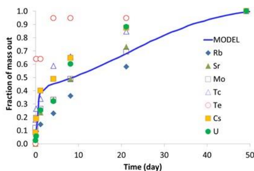
Figure 8: Experimental laboratory data (González-Robles, 2011) of radionuclide release from SNF pellet (normalised to unity) and model prediction assuming that 40% of total tracer mass is initially associated with “macro cracks”.
