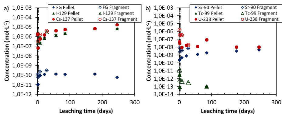
Figure 2: Concentration as a function of leaching time in cladded pellet and fragment experiments: a) ^{129}\text{I} , ^{137}\text{Cs} and normalized content of FG (Xe+Kr); b) ^{90}\text{Sr} , ^{99}\text{Tc} and ^{238}\text{U} .
