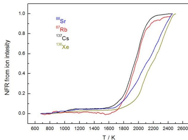
Figure 3. Normalized fractional release of selected fission products determined from the ion intensities measured by KEMS.
