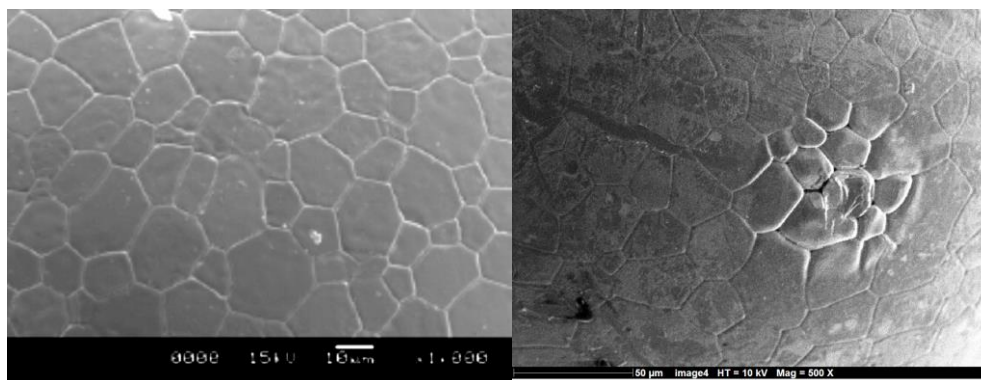
Figure 3: SEM pictures of the surface of a nonirradiated UO 2 particle (left) and of a corroded UO 2 particle (right).
