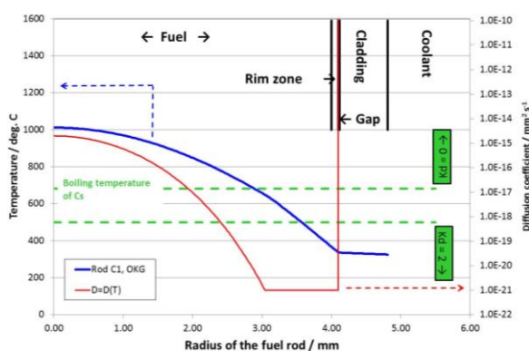
Figure 7: Profiles of temperature and diffusion coefficient over the radius of the C1 pellet.
