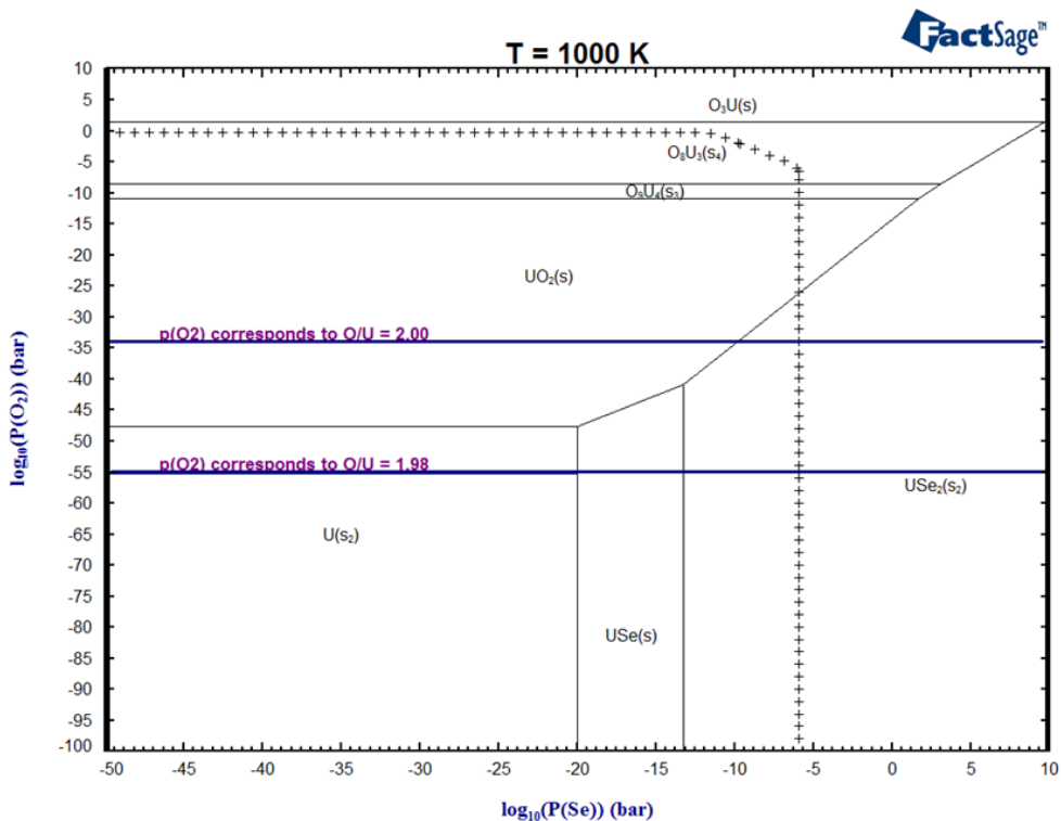
Figure 2: Predominance phase diagram of the Se-U-O system calculated for 1000 K.
