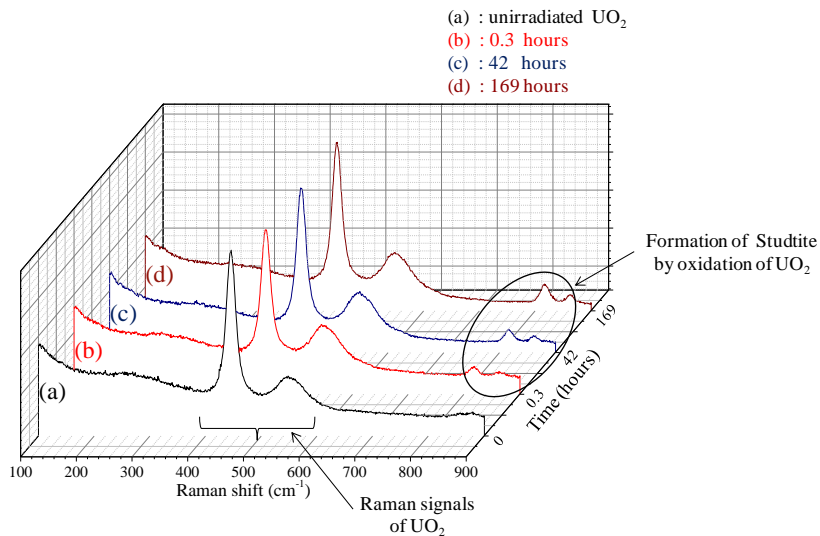
Figure 1: Raman spectra of unirradiated UO_2 ((a)) and a sample irradiated at 8.73 kGy under open atmosphere ((b), (c) and (d)). The spectra (b), (c) and (d) are obtained 0.3, 42 and 169 hours after contact with the irradiated solution.
