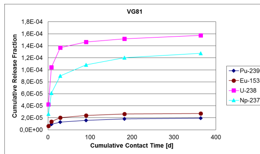
Figure 8: Release rates of 239 Pu, 153 Eu, 238 U and 237 Np sample VG81.
