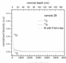
Figure 4 Depth profile for 18 O and 12 C (normalized to 16 O) in reducing condition [Marchetti 2013].
