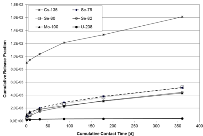
Figure 2: Cumulative release fraction of 79 Se and selected radionuclides from the fragment leaching of sample 5A2.
