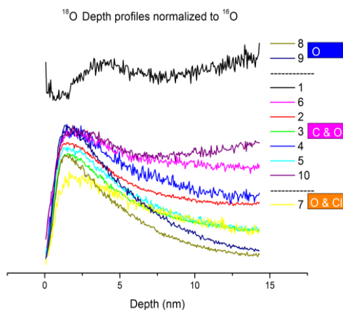
Figure 5: A posteriori depth profiles of selected local ROIs show significantly different diffusivity of ^{18}\text{O} . The ROIs were defined looking at the uneven distribution of ^{18}\text{O} at a nominal depth of 15 nm.
