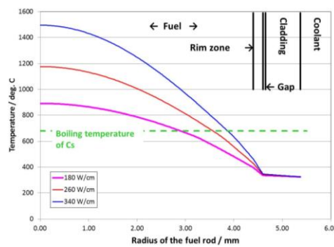
Figure 5: Calculated temperature profiles of a UO 2 pellet in a fuel rod under irradiation.
