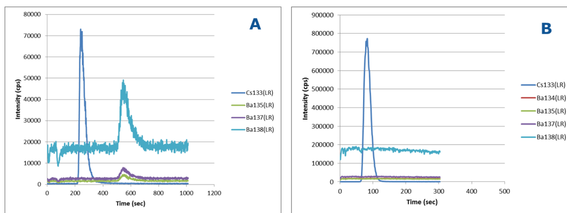
Figure 5: Cs and Ba separation using CG12A, injection volume 100 µL (A) and CG5A, injection volume 250 µL (B) coupled to FAST-ICP-MS. Natural Cs and Ba concentration is 1 ng/g.
