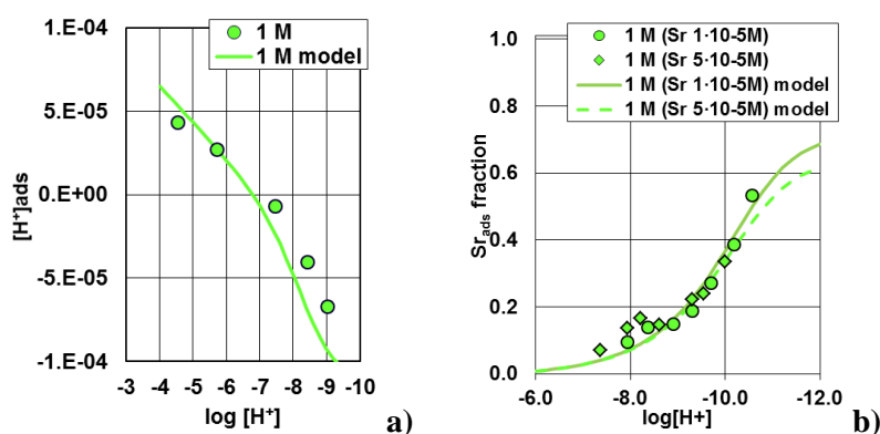
Figure 1. a) H^+ adsorption onto FeOOH(s) surface as a function of pH in 1M NaCl system, b) fraction of Sr adsorbed onto FeOOH(s) in 1M NaCl system (solid line 1 \cdot 10^{-5} M Sr), dashed line 5 \cdot 10^{-5} M Sr).
