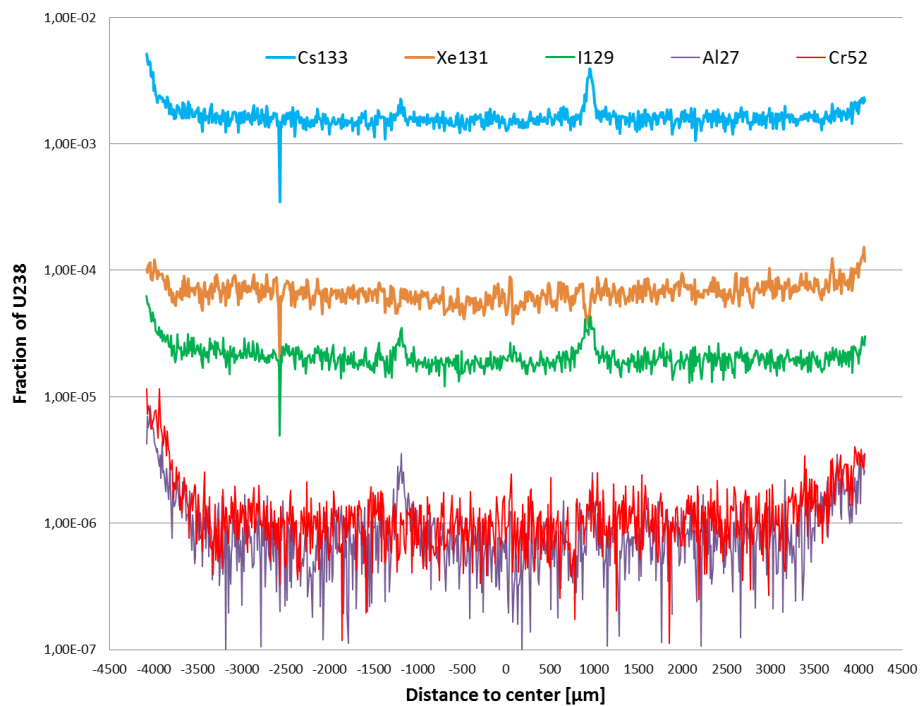
Figure 3: Ablation profiles on 5A2 along the red dashed track in Figure 2 (60 \mu\text{m} beam).
