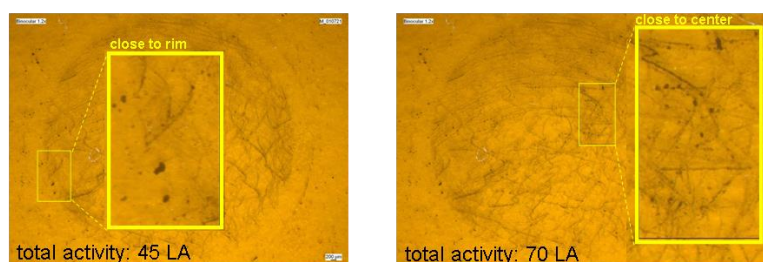
Figure 1: Sample preparation for XANES measurements of the Leibstadt spent fuel. See text for explanation.
