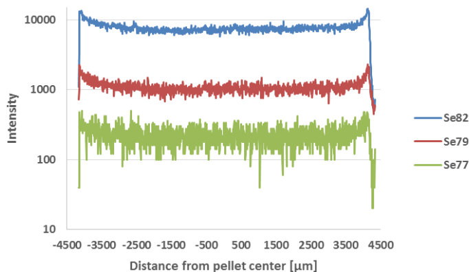
Figure 15: ^{82}\text{Se} , ^{79}\text{Se} and ^{77}\text{Se} ablation profiles on sample 5A2 (60 \mu\text{m} beam).
