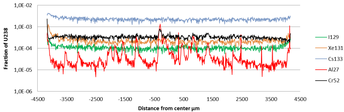
Figure 8: Ablation profiles on sample C1 along the track marked 1 in Figure 7 (60 \mu\text{m} beam).
