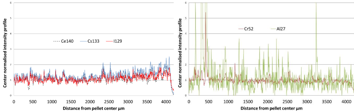
Figure 11: Ablation profiles on C1 in the fine track between 1 & 3 in Figure 7 (10 \mu\text{m} beam).
