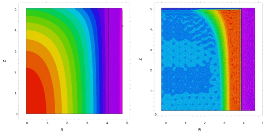
Figure 8: Contour of the calculated temperature in the CI rod (red: highest, magenta lowest). File “rod CI Studsvik_b.pde”.
