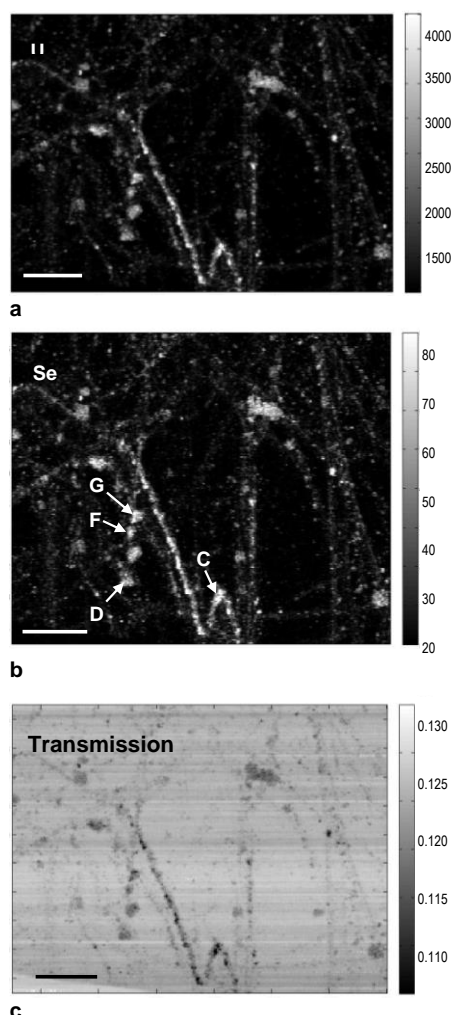
Figure 3: Micro-XRF maps of U (a) and Se (b) fluorescence signals, and transmitted intensity map (c) obtained from a section of a dispersed Leibstadt UO 2 spent fuel sample. Letters and arrows in Figure 3 b denote fuel particles where Se K-edge micro-XANES spectra were recorded. Grey-coded scales represent detector counts (a, b) and voltages of the diode used to measure the transmitted signal (c).
