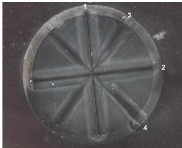
Figure 7: Overview of additive sample C1 after laser ablation.
