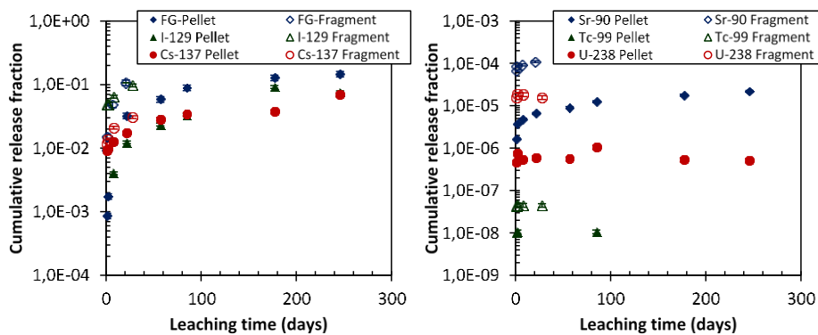
Figure 3: Cumulative release fraction as a function of leaching time in cladded pellet and fragment experiments: (left) FG ( Xe+Kr ), ^{129}I and ^{137}Cs ; (right) ^{90}Sr , ^{99}Tc and ^{238}U .
