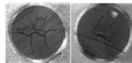
Figure 1. Cross section of spent fuel pellets used in leaching experiments
