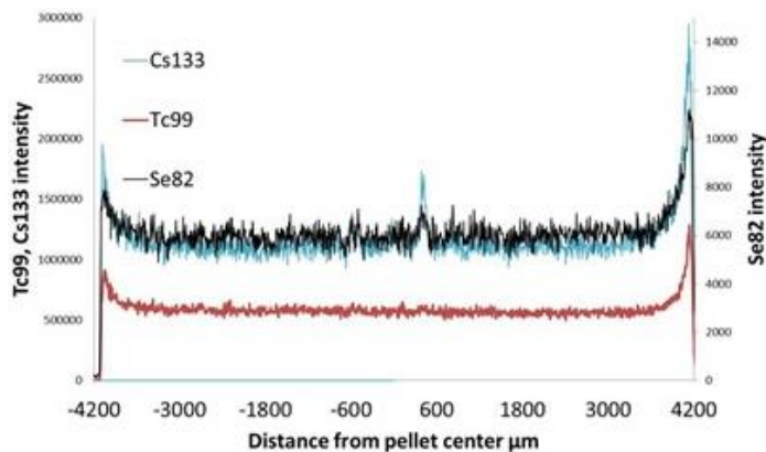
Figure 1: Studsvik profiles of Cs, Tc and Se in a Al/Cr doped UO 2 rod C1 (Tentative Se-identification C1).
