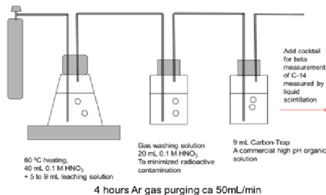
Figure 2: Schematic picture of CO 2 separation method.
