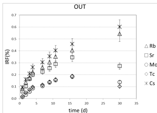
Figure 14: IRF as a function of time for the OUT powder experiment.
