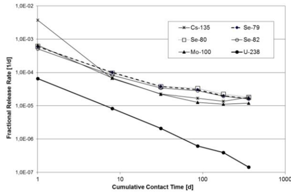
Figure 5: Release rates of ^{79}\text{Se} and selected radionuclides from the fragment leaching of sample C1.
