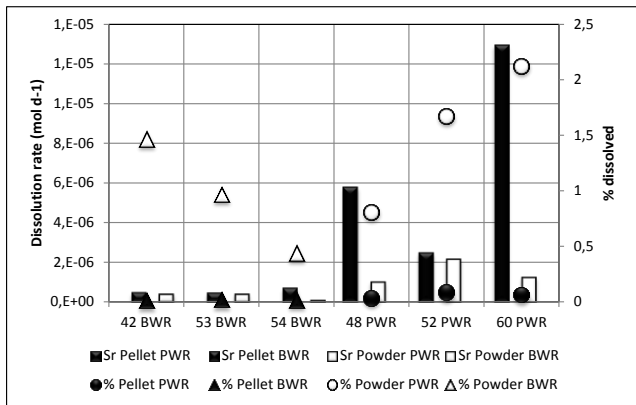
Figure 6: Results for Sr for the different fuel samples studied.
