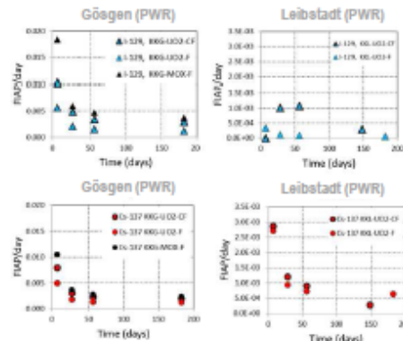
Fig. 4: Calculated release rates (FIAP/day) for ^{137}Cs and ^{129}I for leaching of Gösgen (left) and Leibstadt (right) samples. See legend and ID codes for sample identification
