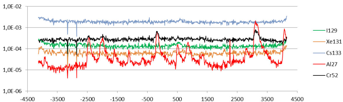
Figure 9: Ablation profiles on sample C1 at the 4 th passage in the track marked 1 in Figure 7 (60 \mu\text{m} beam).
