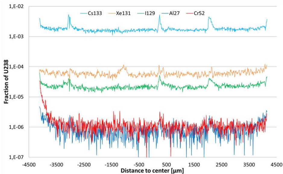
Figure 4: Ablation profiles on 5A2 along the green track in Figure 2 (60 μm beam).
