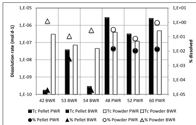
Figure 4: Results for Tc for the different fuel samples studied.
