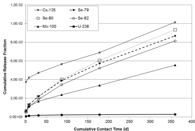
Figure 4: Cumulative release fraction of 79 Se and selected radionuclides from the fragment leaching of sample C1.
