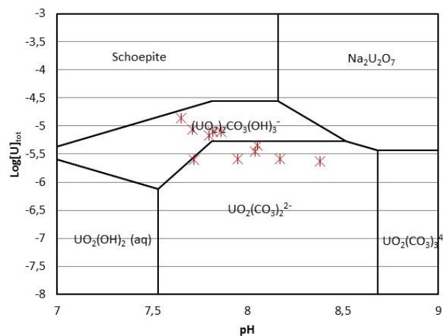
Figure 2: Speciation diagram of uranium in the studied experimental conditions (NEA and CHES databases were used for the calculation). Measured uranium concentrations for each sample in the experiments with the pellet are also included.
