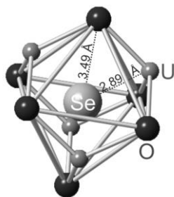
Figure 8: Polyhedral representation of Se-coordination environment resulting from geometrical optimization of a Leibstadt SNF spectrum (“spot 5”) obtained via FDMNES / FitIt calculation.
