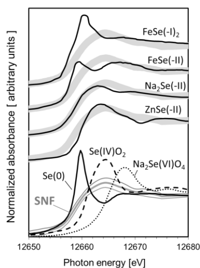
Figure 5: Average smoothed Se K-edge \mu -XANES spectra from all measurements obtained from the spent fuel particles (SNF, thick grey line) and envelope defined by the standard deviation of all individual spectra (thin grey lines or shading) compared with the spectra of reference compounds.
