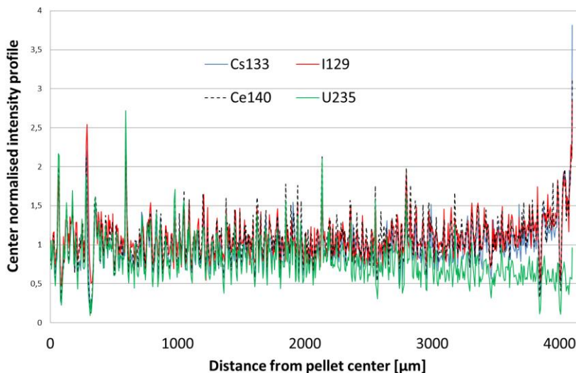
Figure 5: Ablation profiles on 5A2 along the yellow dotted track in Figure 2. (10 μm beam).
