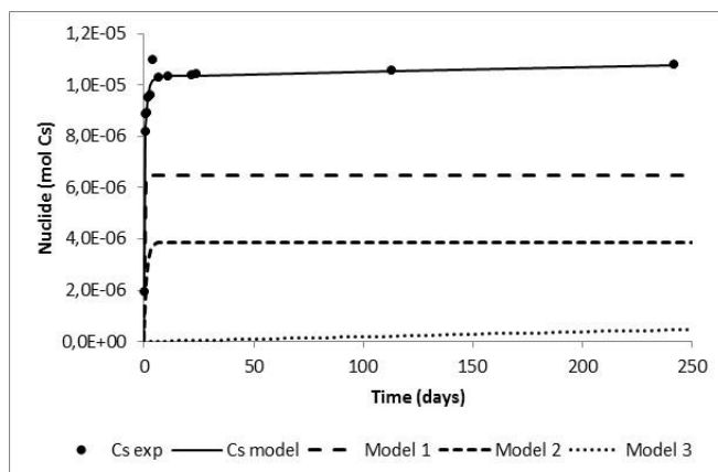
Figure 2: Example of Cesium fitting from static experiments using a cladded fuel segment (González-Robles, 2011). See explanations of the different models in the text.
