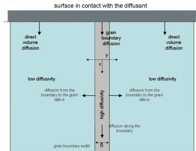
Figure 1: Model of lattice and grain boundary diffusion (Fisher, 1951).
