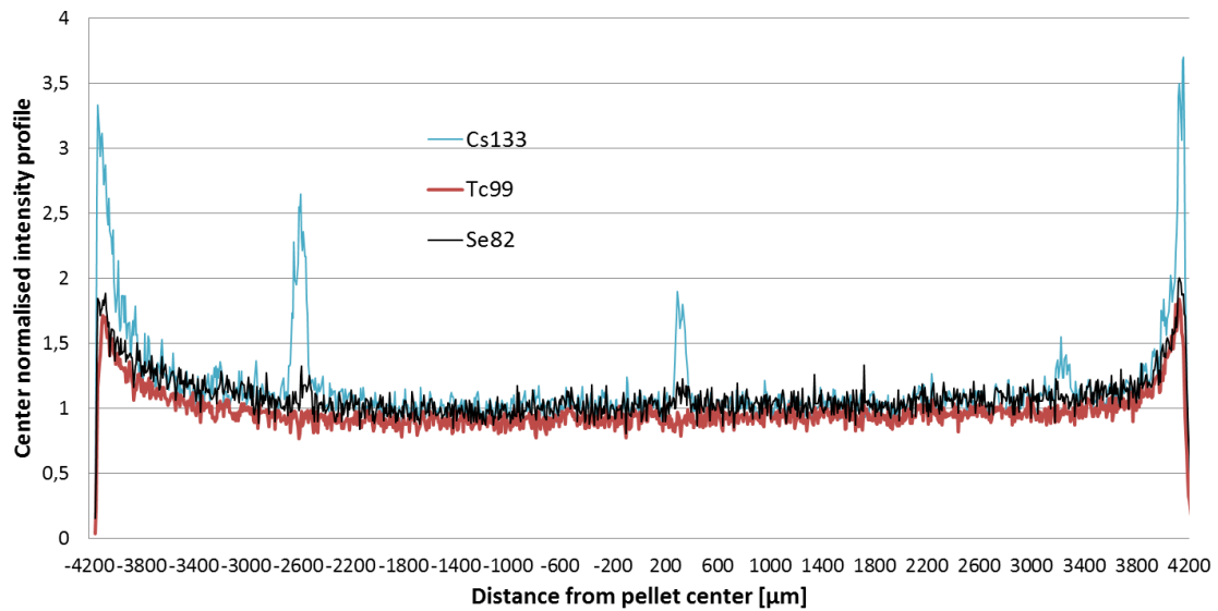
Figure 6: Normalised intensity profiles on 5A2 (60 µm beam) of ^{133}\text{Cs} , ^{99}\text{Tc} and ^{82}\text{Se} .
