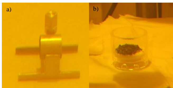
Figure 1: a) Ti sample holder with cladded pellet; b) glass sample holder containing SNF fragments.
