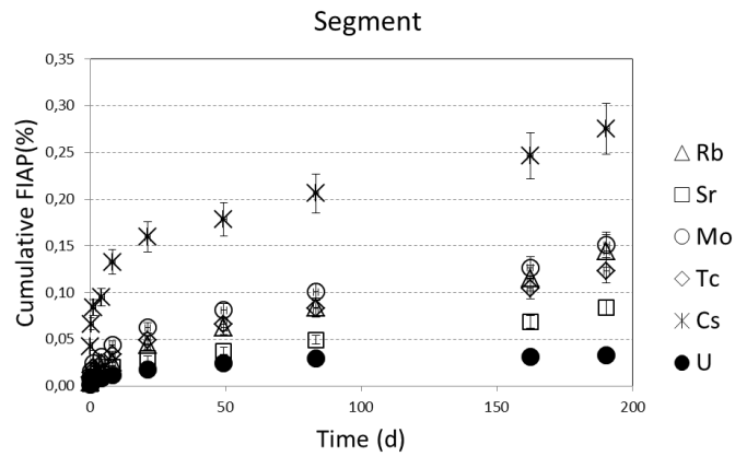
Figure 6: Cumulative FIAP(%) vs time. Experiment carried out with the segment.
