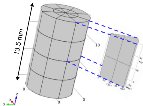
Figure 2: The Reference Pellet with idealised crack pattern (left) and a 1/16 th section selected (based on symmetry criteria) for calculations (right). Pellet dimensions are height = 13.5 mm, diameter = 8.19 mm.
