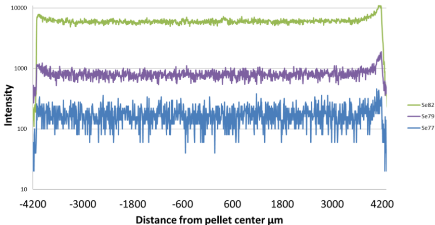
Figure 13: ^{82}\text{Se} , ^{79}\text{Se} and ^{77}\text{Se} ablation profiles on sample C1 (60 \mu\text{m} beam).
