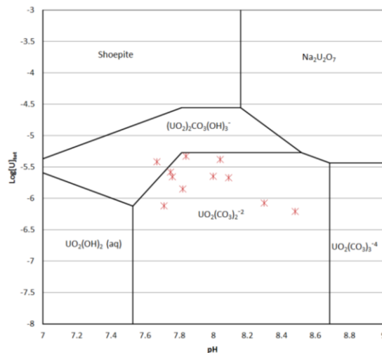
Figure 8: Predominance diagram of main uranium species present in our system. Symbols represent our experimental data.
