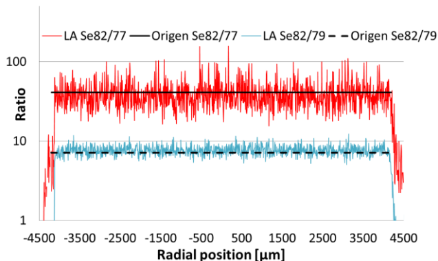
Figure 14: Comparison of Se isotope ratios from LA and pellet average values calculated by the Origen code, sample C1 (60 \mu\text{m} beam).
