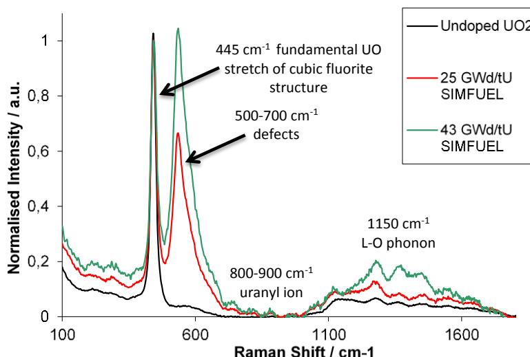
Figure 1: Effect of Fuel Burnup on Raman Spectra.
