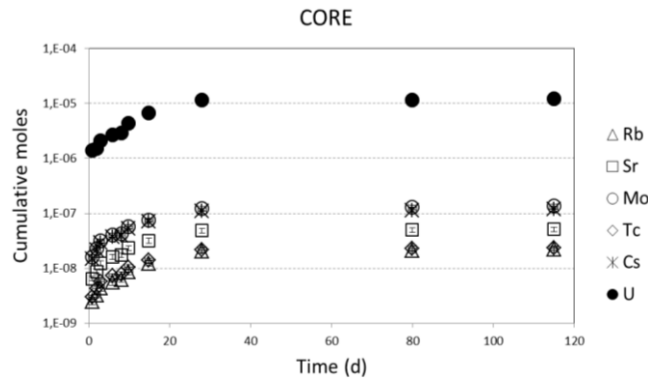
Figure 4: Elemental cumulative moles vs time. Experiment carried out with powder from the center (CORE) of the SNF.
