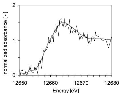
Figure 4: Typical example of a raw (black thin line) and smoothed (grey thick line) Se-K edge XANES spectrum from the Leibstadt spent fuel sample (location C, see Figure 3 b).
