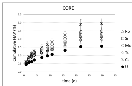
Figure 10: Cumulative FIAP as a function of time for the CORE powder experiment.
