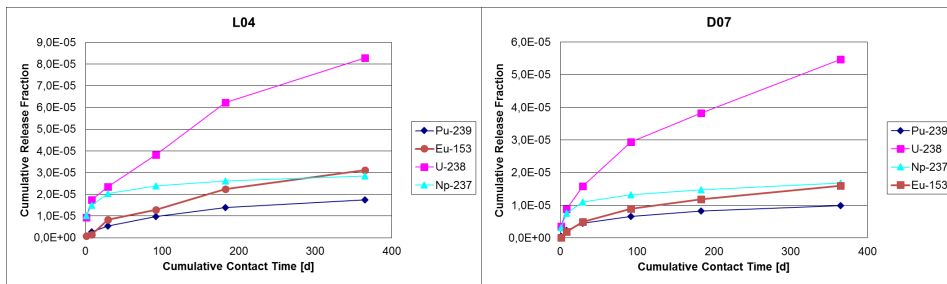
Figure 6: Release rates of 239 Pu, 153 Eu, 238 U and 237 Np sample L01 and D07.
