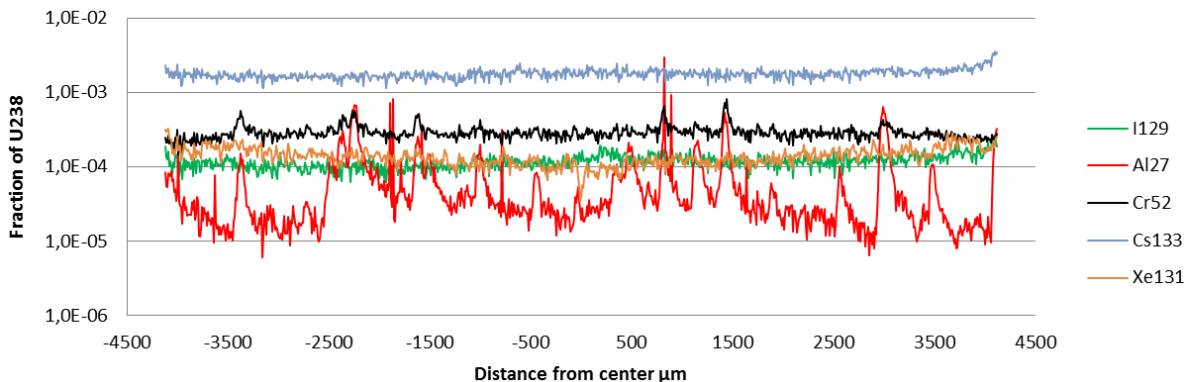
Figure 10: Ablation profiles on sample C1 along the track marked 2 in Figure 7 (60 \mu\text{m} beam).
