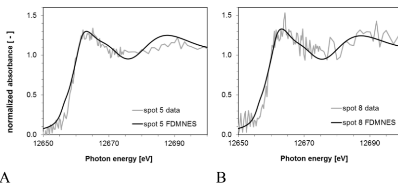
Figure 7: Fits of Se K-edge spectra collected at two distinct spots in the Leibstadt spent fuel sample through geometrical optimization of theoretical XANES.
