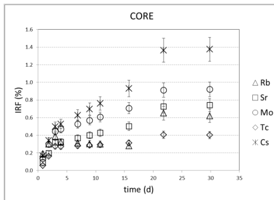
Figure 13: IRF as a function of time for the CORE powder experiment.
