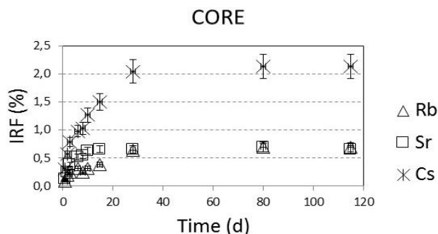
Figure 10: IRF(%) vs. time. Experiment carried out with powder from the centre (CORE) of the SNF.
