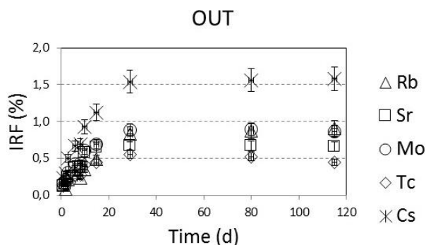
Figure 11: IRF(%) vs. time. Experiment carried out with powder from the periphery (OUT) of the SNF.
