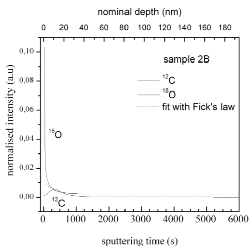
Figure 10: Depth profile for ^{18}\text{O} and ^{12}\text{C} (normalized to ^{16}\text{O} ) in reducing condition (Marchetti, 2013).
