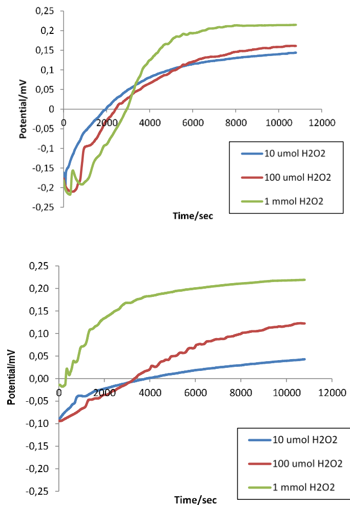
Figure 3: Open Circuit Potentials of \text{UO}_2 in anoxic modified simplified Groundwater ( 0.01 \text{ M NaCl} & 0.002 \text{ M NaHCO}_3 and 43 GWd/ t_U SIMFUEL in anoxic modified simplified groundwater.
