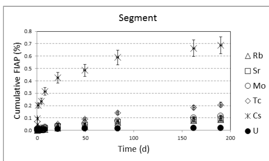
Figure 9: Cumulative FIAP as a function of time for the pellet experiment.
