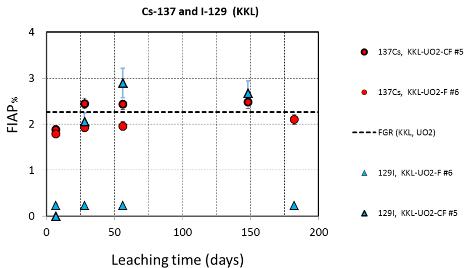
Figure 2: Cumulative percentages of 137 Cs and 129 I inventories in the aqueous phase (FIAP%) as a function of leaching time for UO 2 fuel samples (± cladding) from the Leibstadt BWR, compared with fission gas release (FGR).
