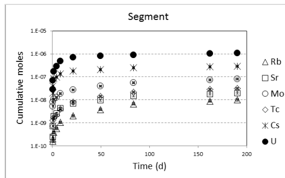
Figure 5: Measured cumulative moles as a function of time for the pellet experiment.
