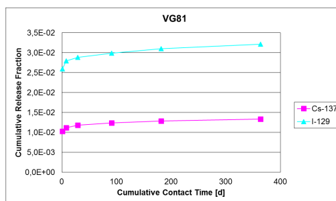
Figure 5: Release rates of 137 Cs and 129 I sample VG81.
