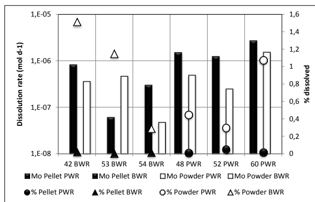
Figure 5: Results for Mo for the different fuel samples studied.
