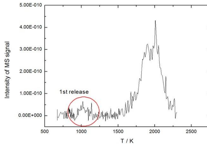
Figure 2: KEMS measurement of ^{137}\text{Cs} released from irradiated \text{UO}_2 fuel before leaching.
