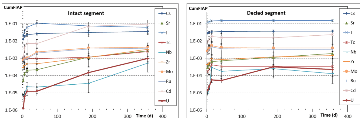
Figure 6: Cumulative FIAP in function of the time for the experiment with the intact segment (left side) and the declad segment (right side).
