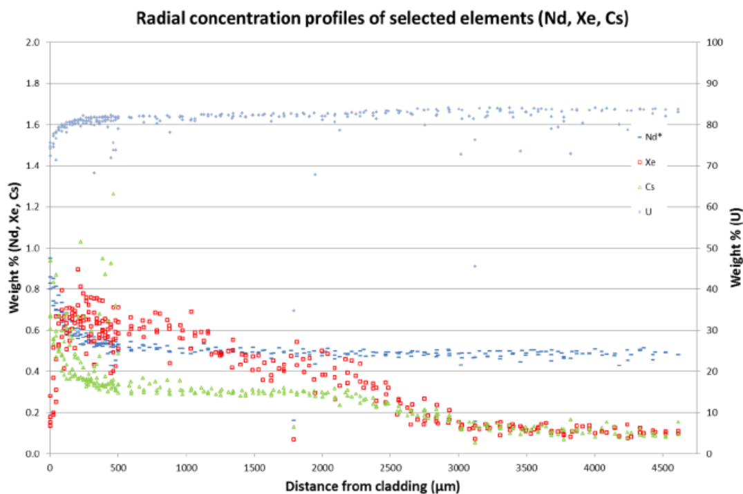
Figure 4: Example of a radial quantitative scans of the spent fuel sample by EPMA.
