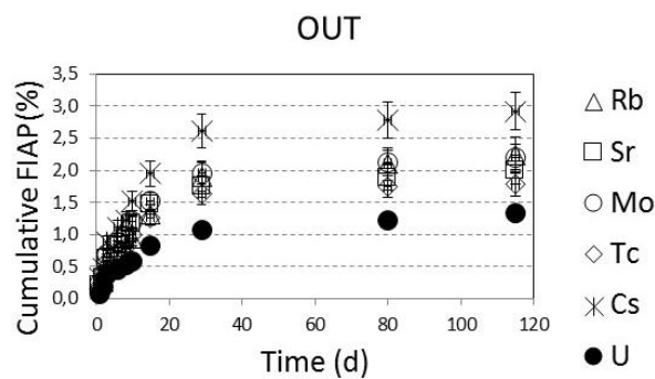
Figure 8: Cumulative FIAP(%) vs time. Experiment carried out with powder from the periphery (OUT) of the SNF.
