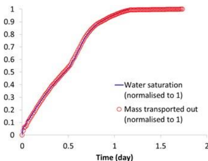
Figure 6: Comparison of the degree of saturation of “macro cracks” (surface integral of water content over all “macro cracks” as a function of time) and the total accumulated mass of a tracer released from the “macro cracks” network and transported to an external reservoir. Both variables are normalised to unity (complete saturation and all radionuclide mass outside the cracks, respectively) to help comparison.
