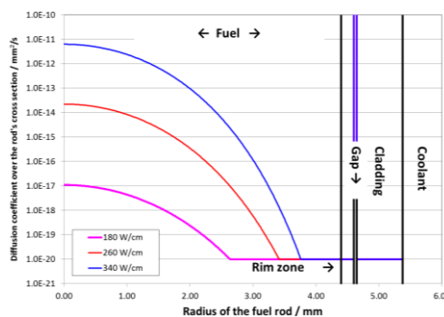
Figure 6: Calculated temperature depending diffusion coefficient profiles in a UO 2 pellet for a fuel rod under irradiation.
