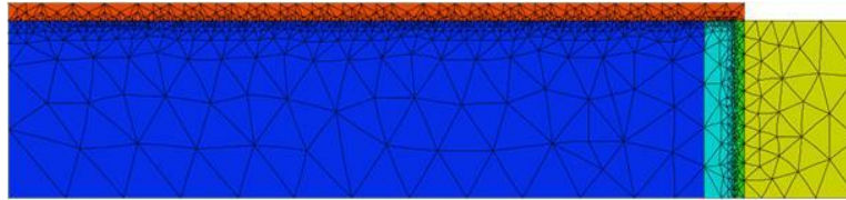
Figure 4: Finite element discretization (R, Z cylinder geometry) of the rod slice. (blue: fuel; turquoise: rim zone; dark green: gap; light green: cladding; red: gap between pellets).
