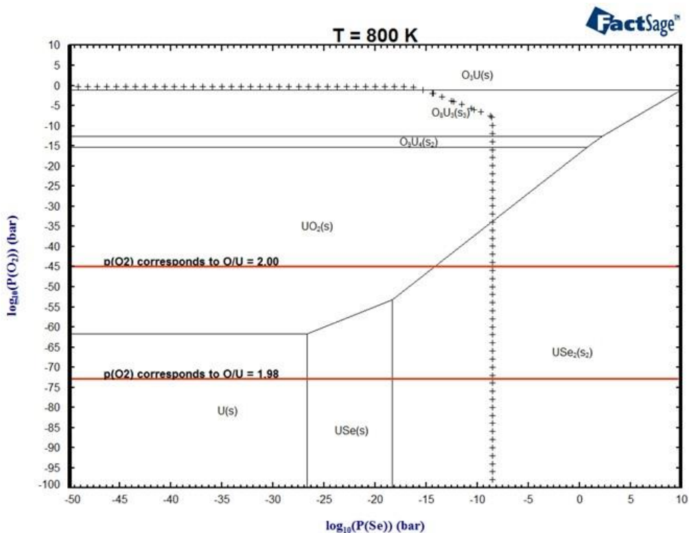
Figure 1: Predominance phase diagram of the Se-U-O system calculated for 800 K.
