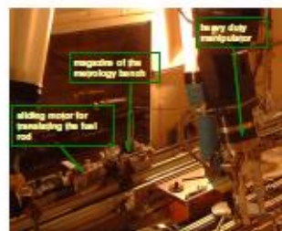
Figure 1 Inside view of the hot cell used for non-destructive testing of spent fuel rods.
