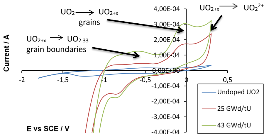
Figure 2: Cyclic Voltammetry of UO 2 , 25 & 43 GWd /t U SIMFUELS, Ar sparged in 0.1 M Na 2 SO 4 .
