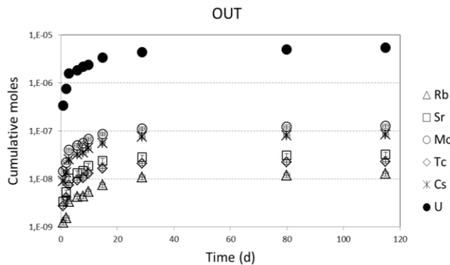
Figure 5: Elemental cumulative moles vs time. Experiment carried out with powder from the periphery (OUT) of the SNF.
