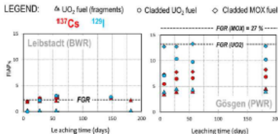
Fig. 3: Fractions of Inventory in the aqueous phase (FIAP) for ^{137}Cs and ^{129}I (in percent) derived from the gamma measurements on the sampled leaching solutions. No correction for matrix dissolution was made.
