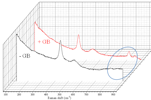
Figure 4: Raman spectra of corroded UO_2 with GB (red) and without GB (black).
