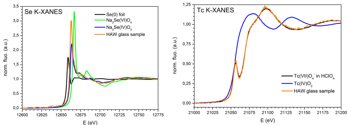
Figure 2: Normalized Se K- (left) and Tc K-XANES spectra of the HAWC glass fragment and corresponding reference spectra.
