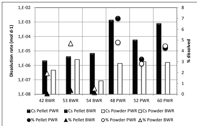
Figure 8: Results for Cs for the different fuel samples studied.
