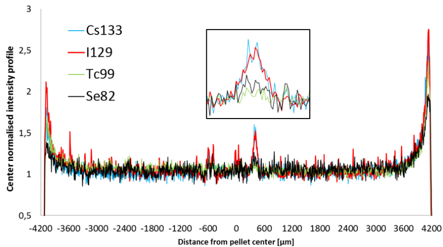
Figure 12: Ablation profiles on sample C1 (60 \mu\text{m} beam).
