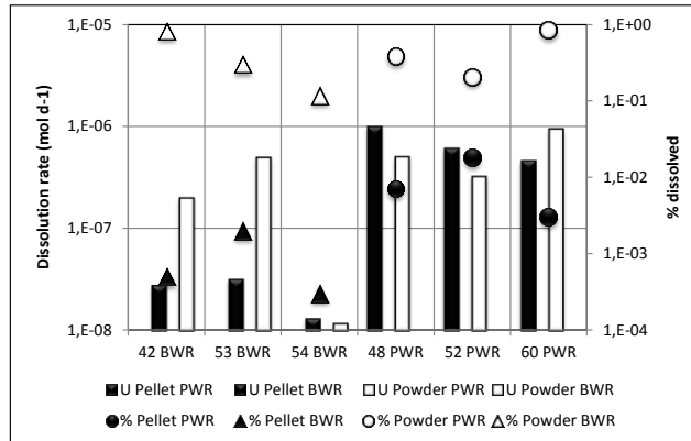
Figure 3: Results for U for the different fuel samples studied.
