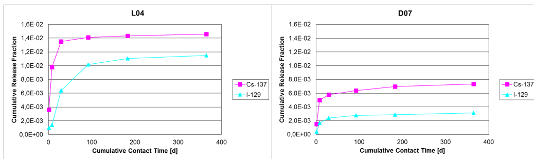
Figure 3: Release rates of 137 Cs and 129 I sample L01 and D07.
