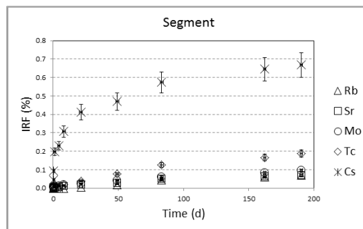
Figure 12: IRF as a function of time for the pellet experiment.
