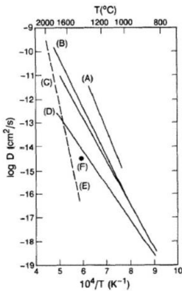
Figure 2: Diffusion coefficient for Xe as function of the temperature.
