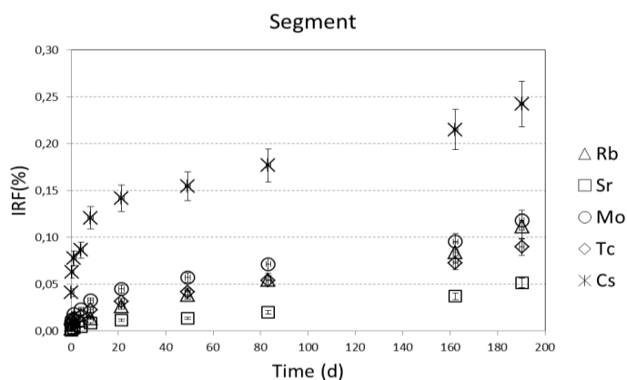
Figure 9: IRF(%) vs. time. Experiment carried out with the segment.
