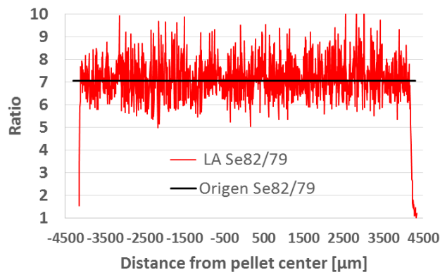
Figure 16: Comparison of ^{82/79}\text{Se} isotope ratios from LA and pellet average values calculated by the Origen code for sample 5A2 (60 \mu\text{m} beam).
