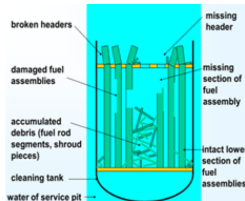
Figure 1: Distribution of damaged fuel in the cleaning tank (Slonszki et al., 2010).
