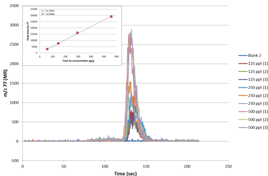
Figure 2: Pre-concentration of Se in nuclear spent fuel analogue samples in a Nobias column at different Se concentrations. \text{Se}(\text{IV}) species.
