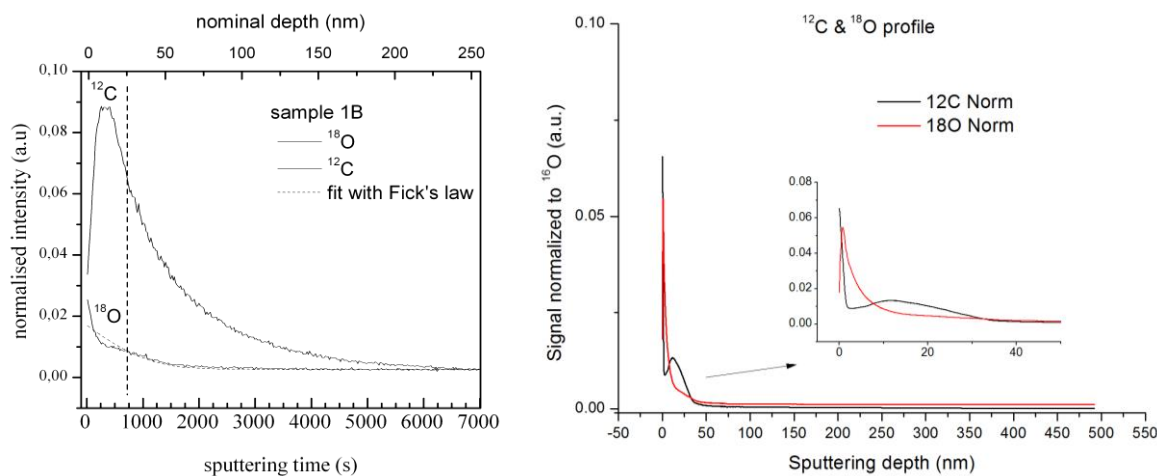
Figure 3: SIMS depth profiles of \text{UO}_2 sample 1B, measured 2010-03-20 (left) and 2014-03-04 (right), with ^{18}\text{O} and ^{12}\text{C} signals normalized to ^{16}\text{O} .
