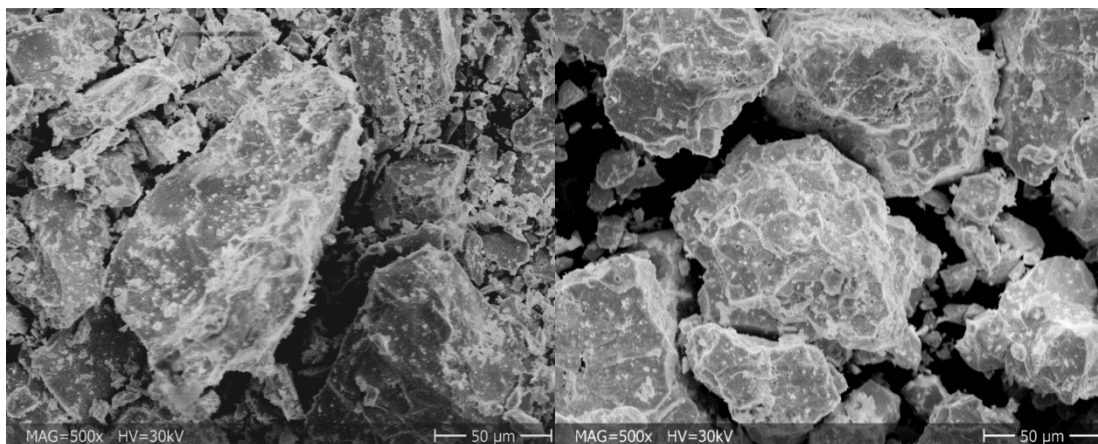
Figure 1: SNF powders taken from the centre, CORE (left), and the periphery of the fuel, OUT (right).
