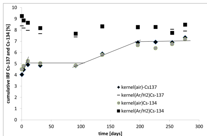
Figure 3: FIAP values for ^{134}\text{Cs} (%) and ^{137}\text{Cs} (%) under oxidic and anoxic/reducing conditions.
