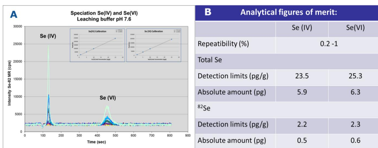
Figure 3: A: Se species elution profiles at different concentrations. B: Analytical figures of merit.
