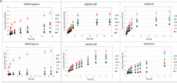
Figure 5. Cumulative FIAP (%) vs time. Experiments carried out with the segment, and the powder sample of both 42BWR and 54BWR fuels.
