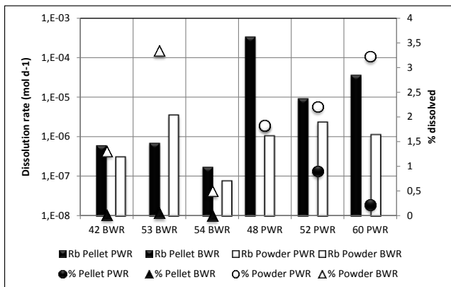
Figure 7: Results for Rb for the different fuel samples studied.
