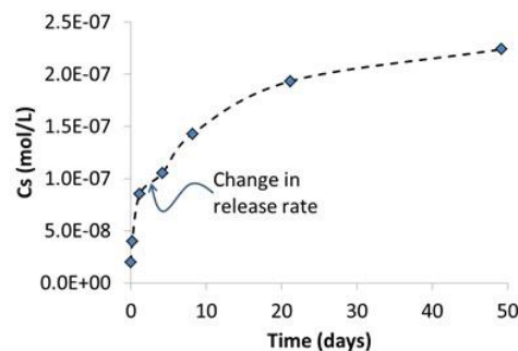
Figure 7: Experimental laboratory data on Cs release from SNF pellet (data of González-Robles (2011)).
