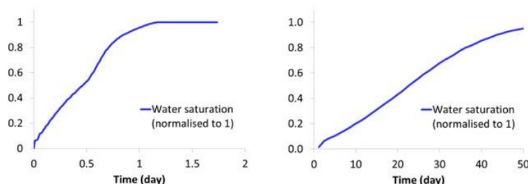
Figure 4: Total water content (surface integral over all “macro cracks” and volume integral over the pellet volume for “macro” and “micro” cracks, respectively), normalised to unity (complete saturation), as a function of time. “Macro cracks” – left, “micro cracks” – right.
