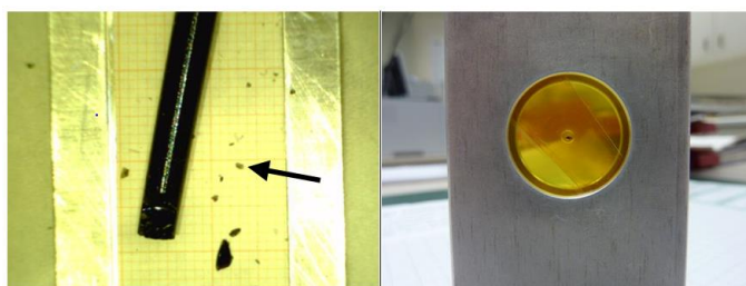
Figure 1: HAWC glass fragment (arrow) selected for investigation at INE-Beamline (left, scale in mm); glass fragment inside a double containment mounted in the sample holder (right) prior to the transport to ANKA.
