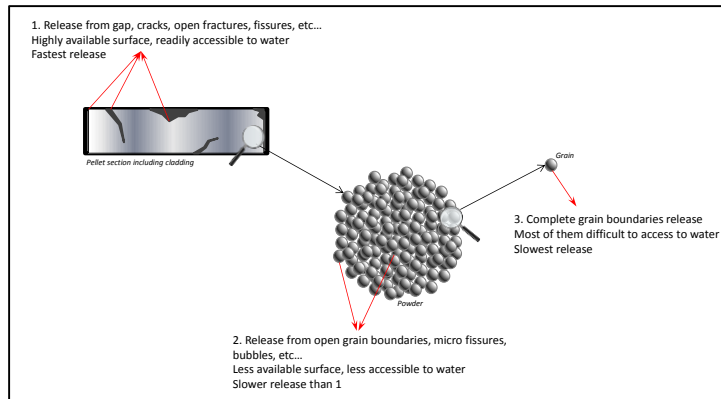
Figure 1: Conceptual description of the experimentally determined release of different radionuclides segregated from the matrix based on sample location, availability to water and sample pretreatment.
