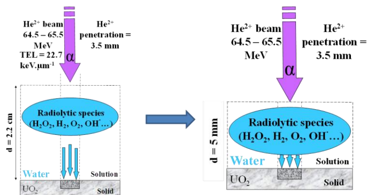
Figure 2: Schematic picture of the variation in the distance between the localized radiolysis of water induced by the He 2+ beam and the UO 2 surface.
