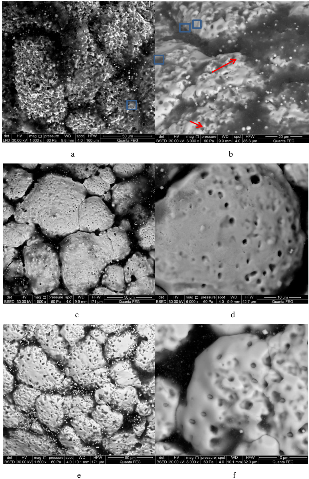
Figure 4: SEM pictures of spent UO 2 kernels: a and b: before leaching; c and d: leaching under oxic conditions; and e and f: leaching under anoxic/reducing conditions.
