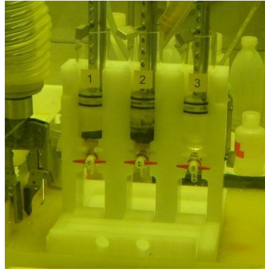
Figure 5: Experimental setup used for the leaching of the spent fuel with an intact segment (1) and a declad segment (2), the column 3 is a blank test.
