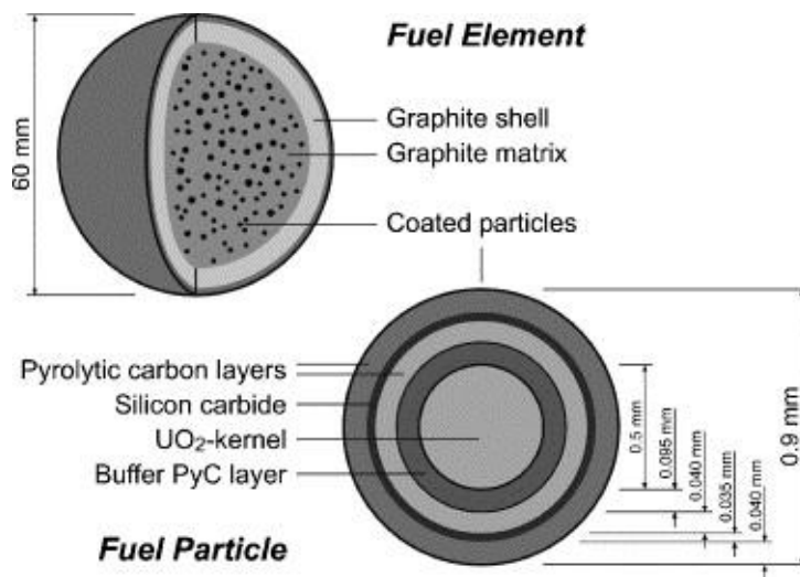
Figure 1: Design of a HTR fuel element and of a TRISO coated fuel particle.
