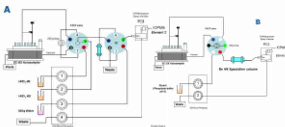
Figure 1 FAST system configurations for pre-concentration and/or separation (A) and speciation analysis (B) purposes
