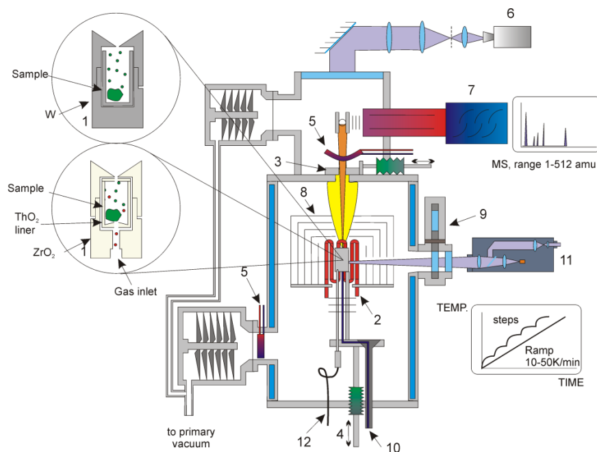
Figure 1: Schematic of the actual KCMS system at ITU. 1: Knudsen cell, 2: heating coil, 3: chopper, 4: lift, 5: LN2 cold trap, 6: camera, 7: mass spectrometer, 8: thermal shields, 9: revolving windows, 10: gas inlet, 11: pyrometer, 12: thermocouple.
