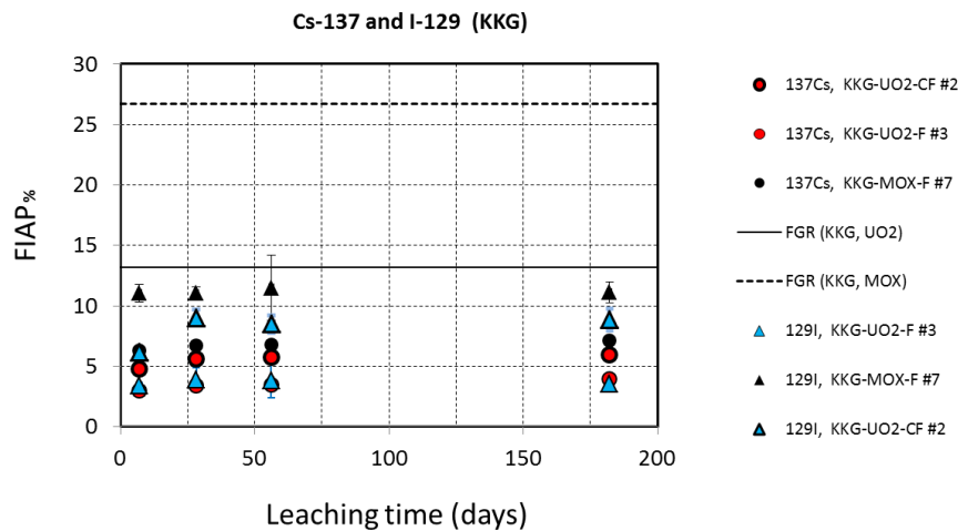
Figure 3: Cumulative percentages of 137 Cs and 129 I inventories in the aqueous phase (FIAP%) as a function of leaching time for UO 2 and MOX fuel samples ( \pm cladding) from the Gösgen PWR, compared with fission gas release (FGR).
